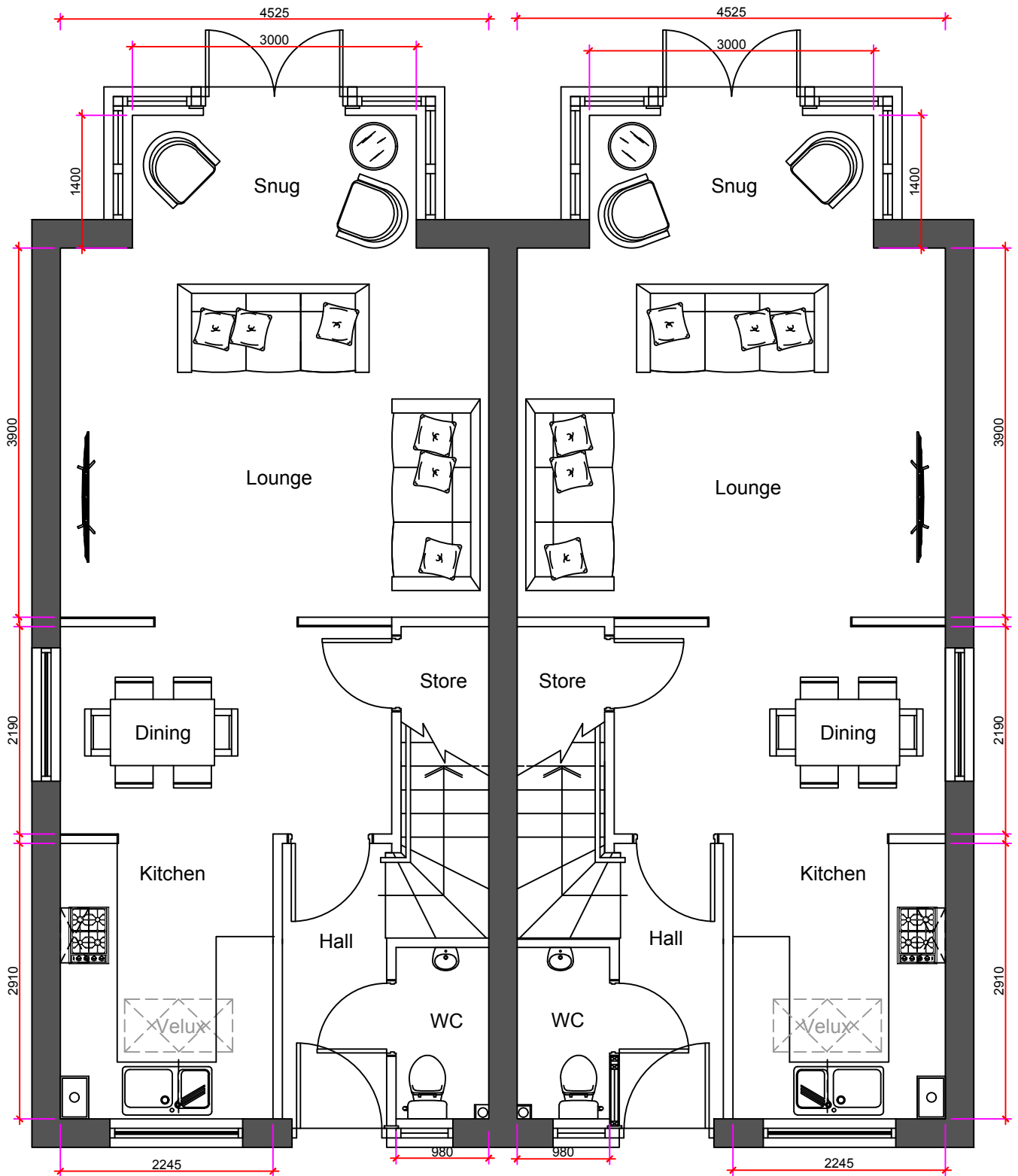
Plot 12 Ground Floor
