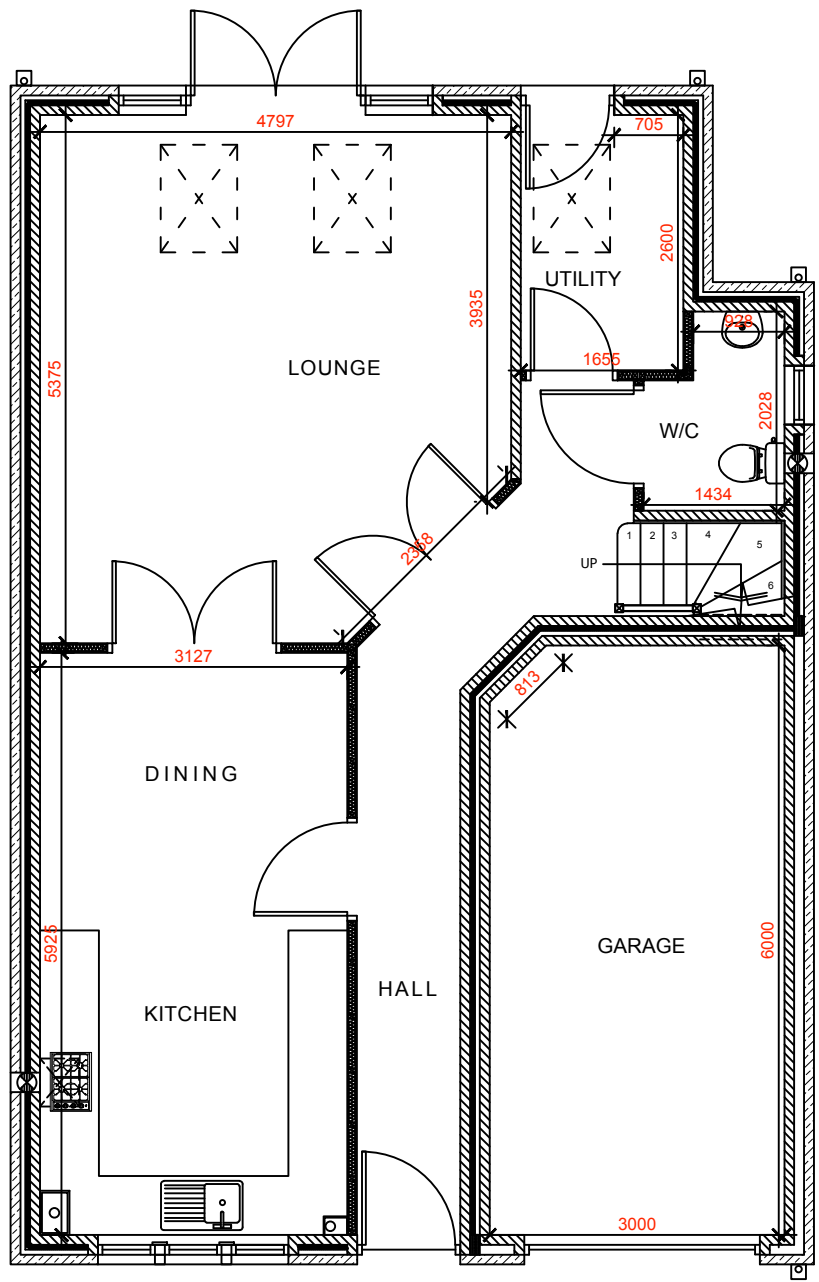
GROUND FLOOR PLOT 1
